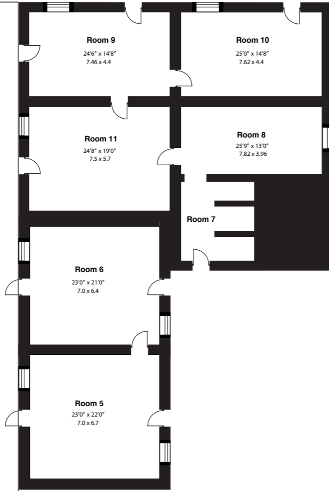
Ground Floor
